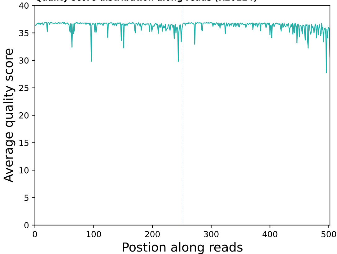
Quality score distribution along reads (R20124)
